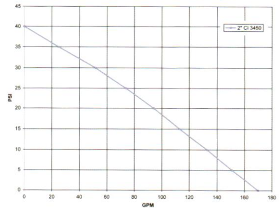
2" Cast Iron Transfer Pumps
